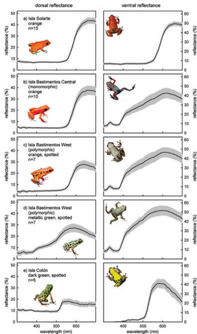
Figure 4. Male reflectance spectra. Curves represent average reflectances of all males used in the experiments. Gray areas indicate between-individual variation (standard errors). Left panels are dorsal reflectance spectra; right panels are ventral reflectance spectra.
