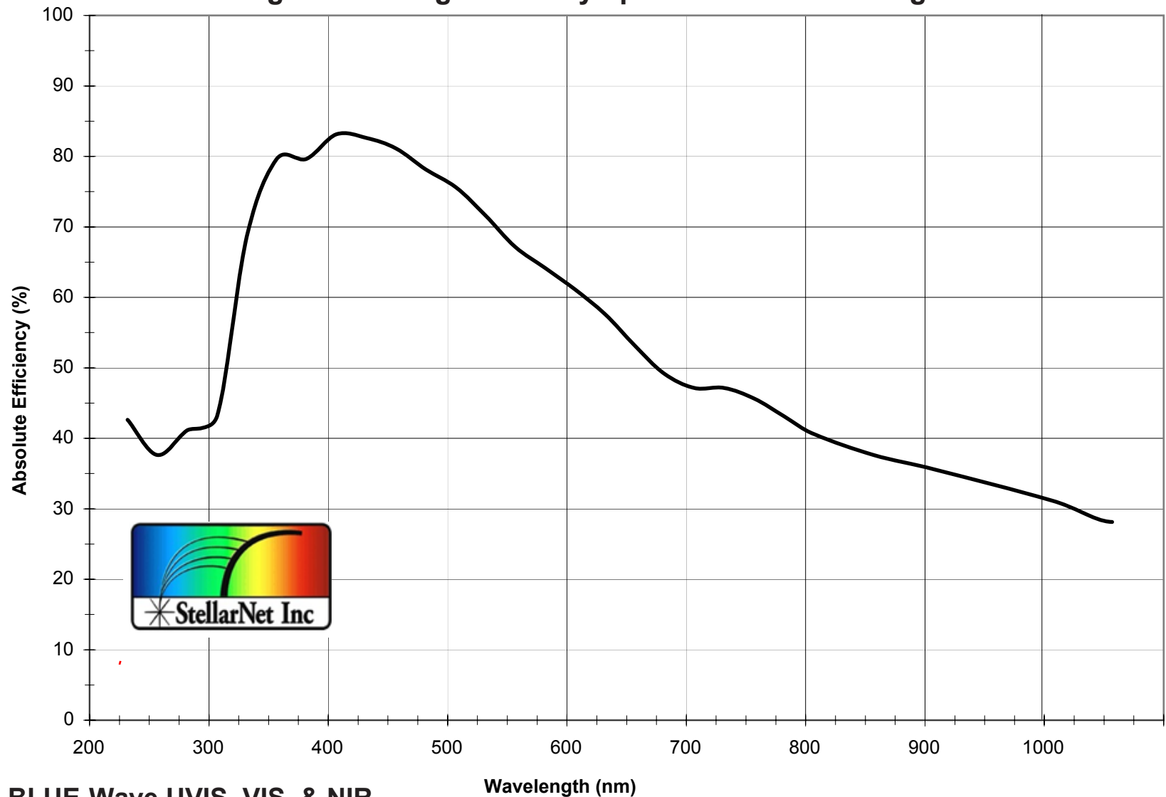
600 g/mm Grating Efficiency optimized for visible light
